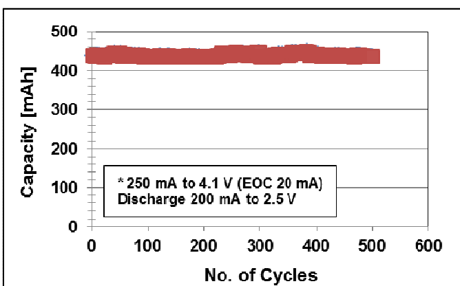
Charge/ Discharge Cycling Performance at RT *
