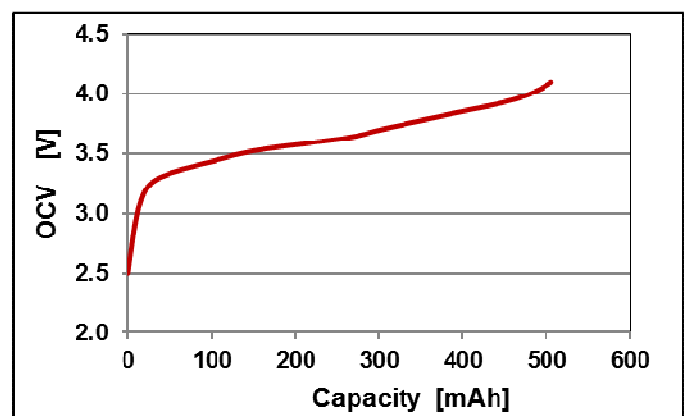
OCV vs. Capacity
